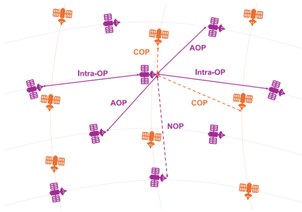
Fig. 6. Example of ISL Topology. The dotted lines represent orbits. The solid and dashed arrows represent persistent links and temporary links, respectively.
